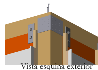
Conector exterior
